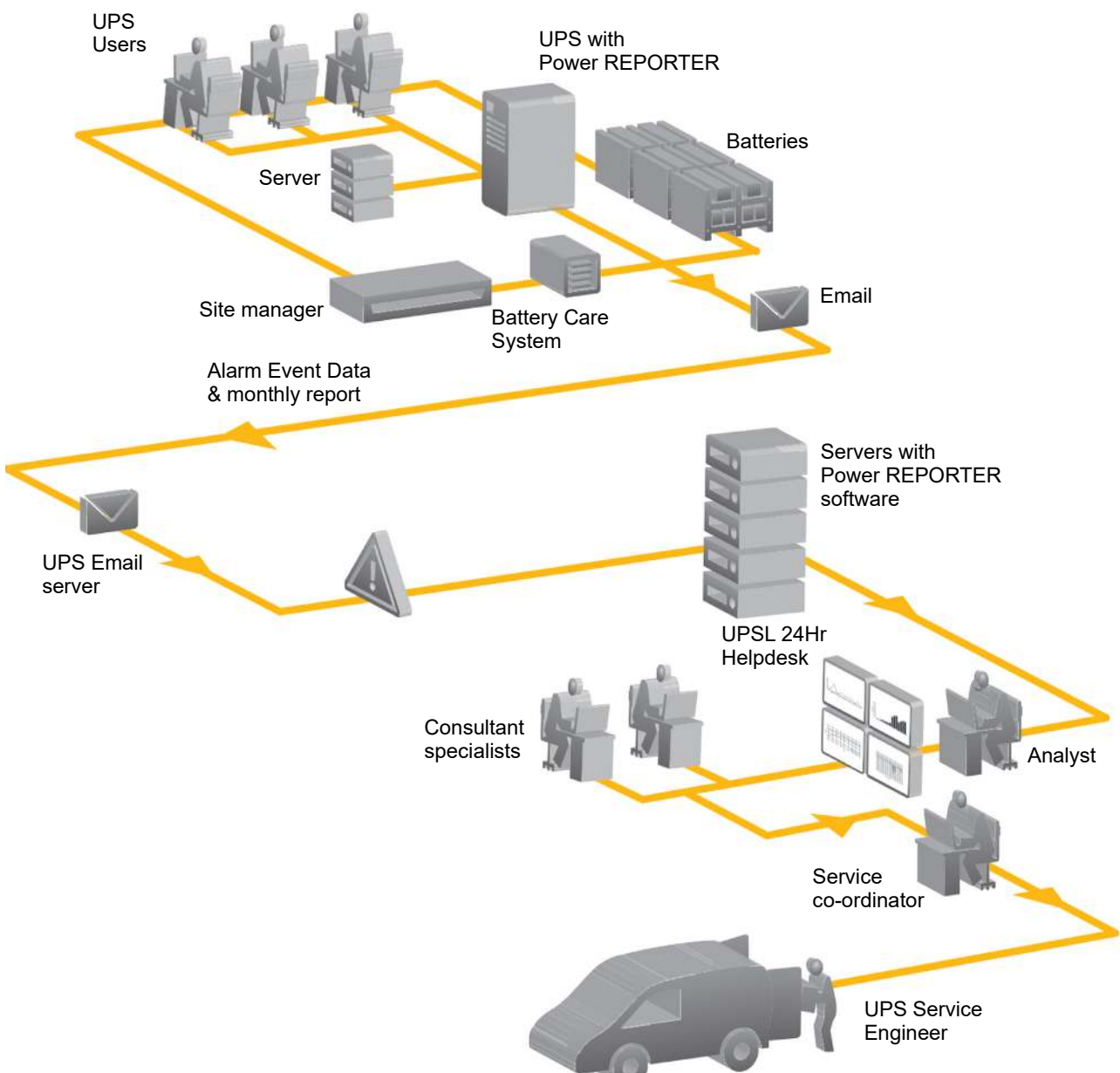
Figure 1 PowerREPORTER operation
