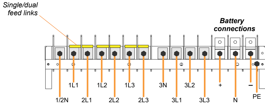
160kVA- 200kVA Power connections
