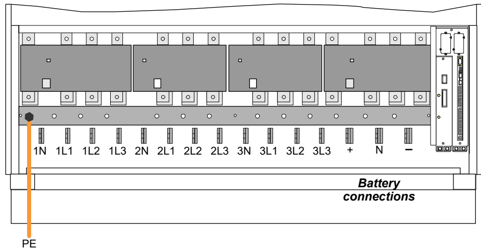
400kVA - 500kVA Power connections
