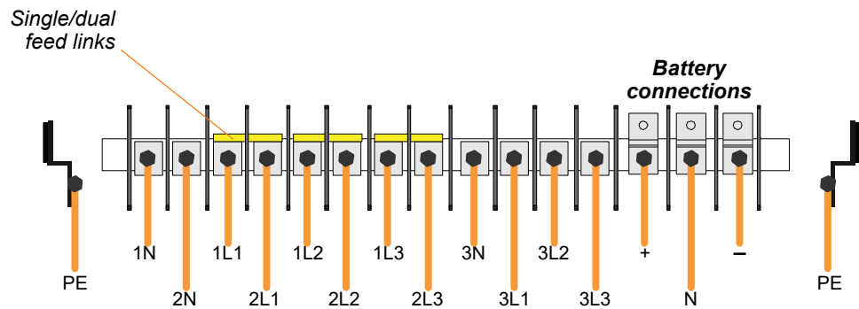
250kVA- 300kVA Power connections
